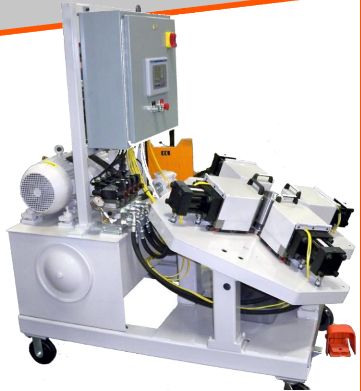
SLOT-400 MACHINE: Puts straight or torca slots in tubes between 3" and 6" diameter
